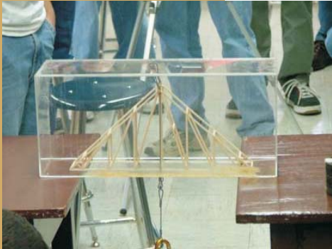
Balsa Wood bridge (truss)
